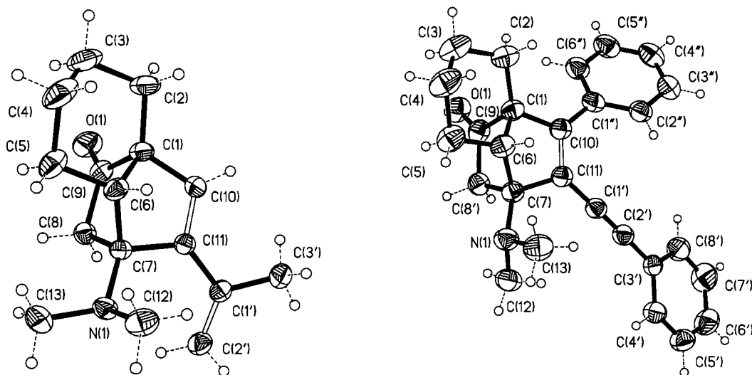
Figure 1. Structures of 5d (left) and 5i (right) in the crystals; 5d : C 16 H 23 NO, monoclinic crystals of space group P 2 1 / c , unit cell dimensions: a = 9.618(2), b = 10.817(2), c = 13.411(3) Å, \beta = 98.75(3)°, V = 1379.0(5) Å 3 , 3405 reflections; 5i : C 27 H 27 NO, triclinic crystals of space group P 1 , unit cell dimensions: a = 10.13(3), b = 15.01(4), c = 15.10(3) Å, \alpha = 99.2(2), \beta = 107.8(2), \gamma = 96.6(2)°, V = 12125(9) Å 3 , 9865 reflections
