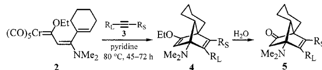
Scheme 2. For details see Table 1
