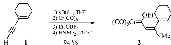
Scheme 1. Preparation of the Fischer carbene complex 2 in a one-pot sequence
