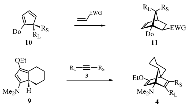
Scheme 4. Regional and facial selectivities in Diels–Alder reactions; Do: electron-donating group; R_L, R_S : larger and smaller substituent; EWG: electron-withdrawing group
