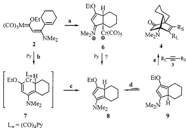
Scheme 3. On the mechanism for the formation of cycloaddition products 4 ; a: 1,5-cyclization; b: 6 \pi -electrocyclization; c: reductive elimination; d: 1,5-hydrogen shift; e: [4+2] cycloaddition
